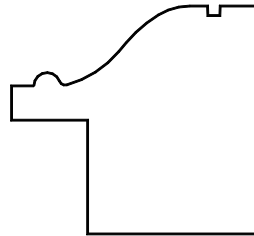
PCP-530 1 1/2"X1 5/8"
